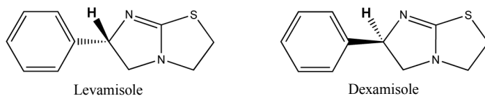
Figure 1 - Structures of levamisole and dexamisole.
