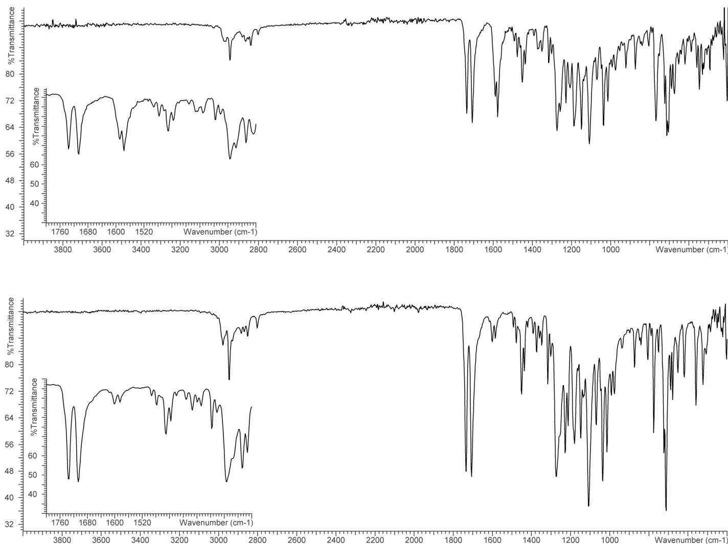
Figure 2 - FTIR spectra of cocaine base/tetramisole base (50:50) mixture (above) and cocaine base after liquid/liquid extraction (below). Inserts of the interfering regions are included for comparison.
