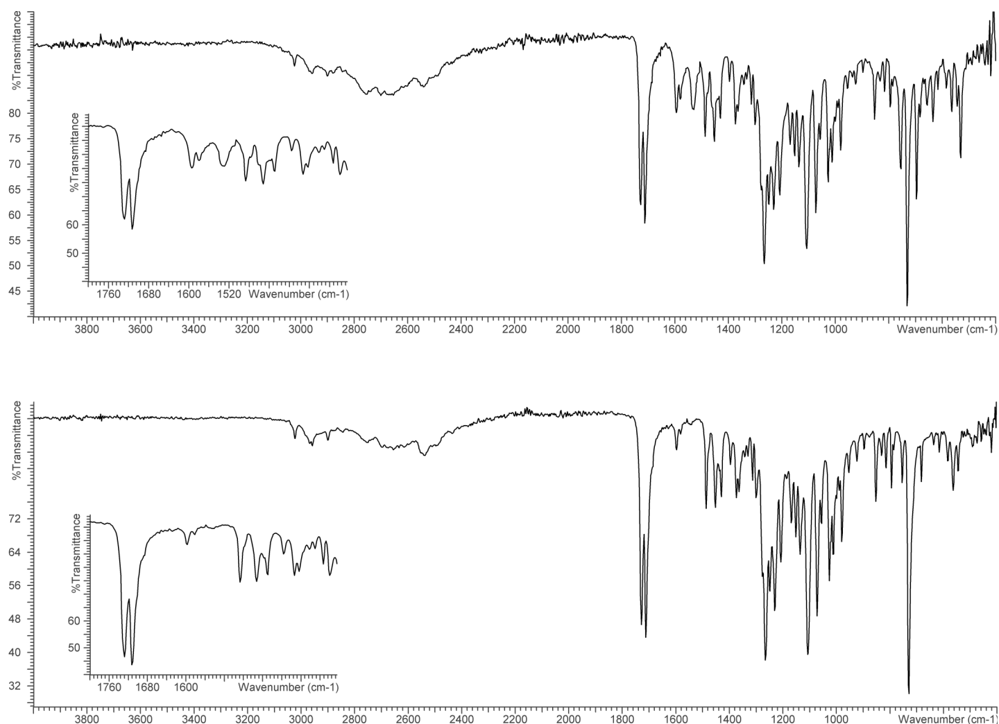
Figure 3 - FTIR spectra of cocaine HCl/tetramisole HCl (50:50) mixture (above) and cocaine HCl after separation via ion pair chromatography (below). Inserts of interfering regions are included for comparison
